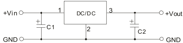
Positive Output Application Circuit
