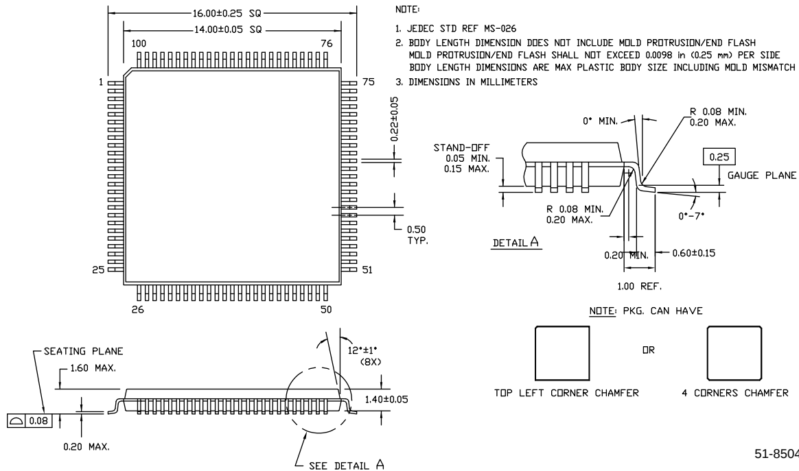
Figure 20. 100-Pin (14 × 14 × 1.4 mm) TQFP
