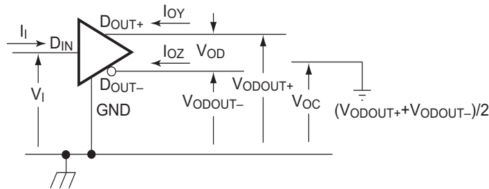
Figure 1. Voltage and Current Definitions
