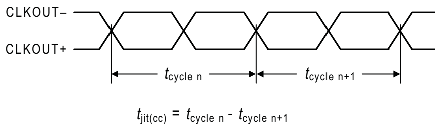
Figure 6. Cycle-to-Cycle Jitter
