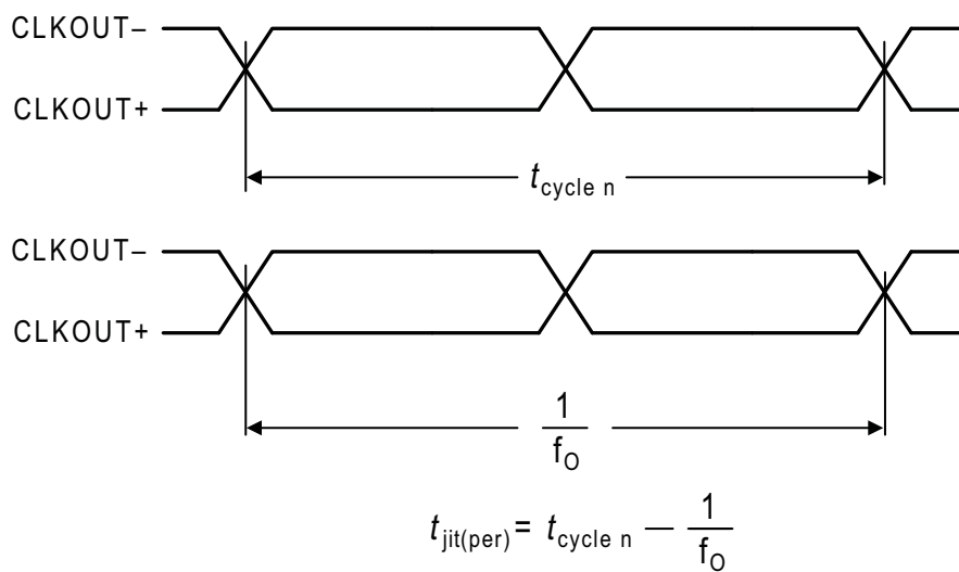
Figure 7. Period Jitter
