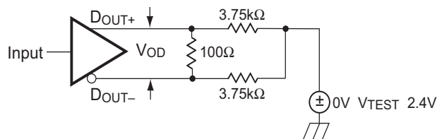
Figure 2. V_{OD} Test Circuit
