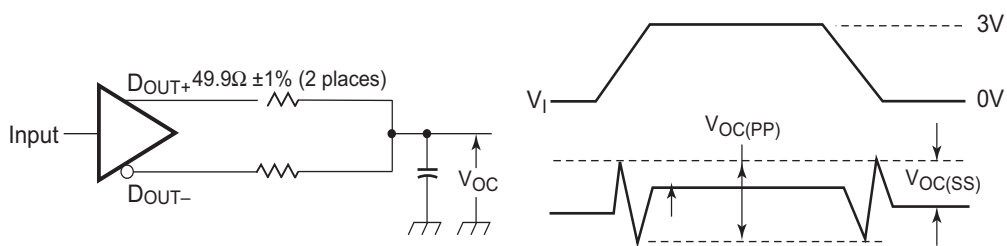
Figure 3. Test Circuit & Definitions for the Driver Common-Mode Output Voltage
