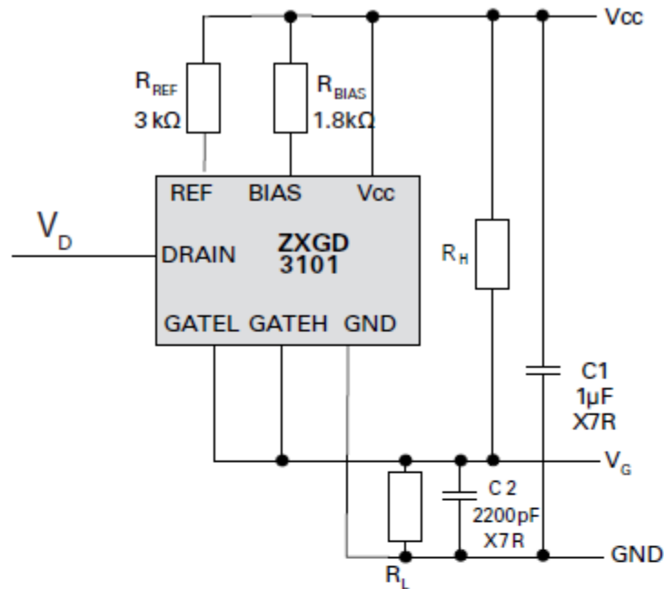
Figure 4: Test circuit
