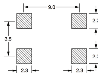
Figure 3) Land Pattern
