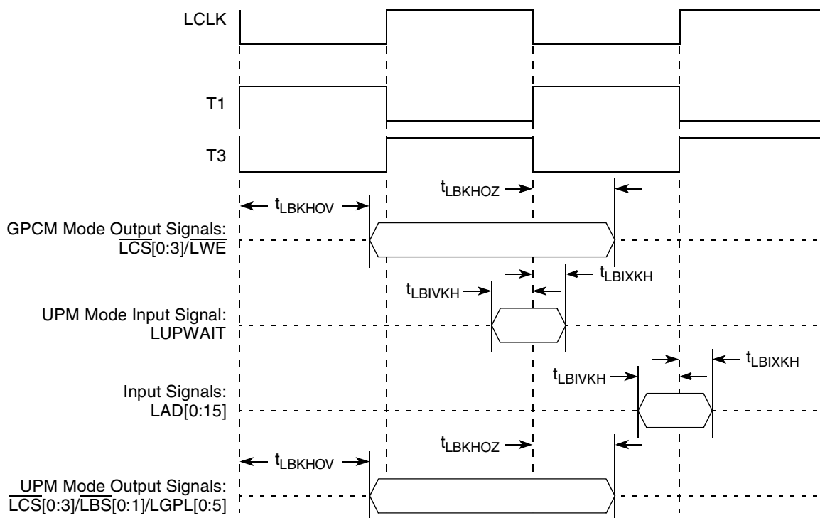
Figure 26. Local Bus Signals, GPCM/UPM Signals for LCCR[CLKDIV] = 2
