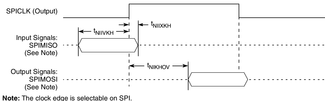
Figure 58. SPI AC Timing in Master Mode (Internal Clock) Diagram
