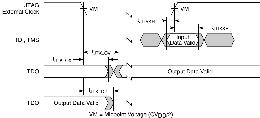
Figure 26. Test Access Port Timing Diagram
