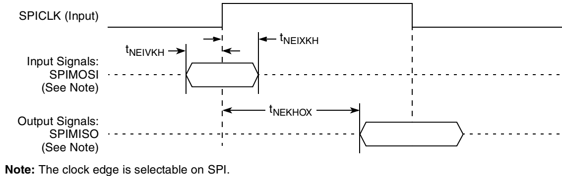
Figure 33. SPI AC Timing in Slave Mode (External Clock) Diagram
