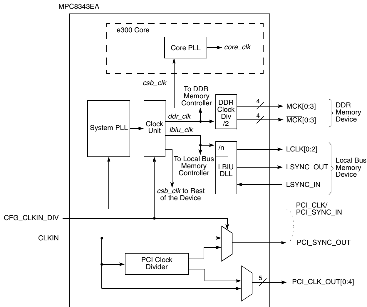
Figure 36. MPC8343EA Clock Subsystem
