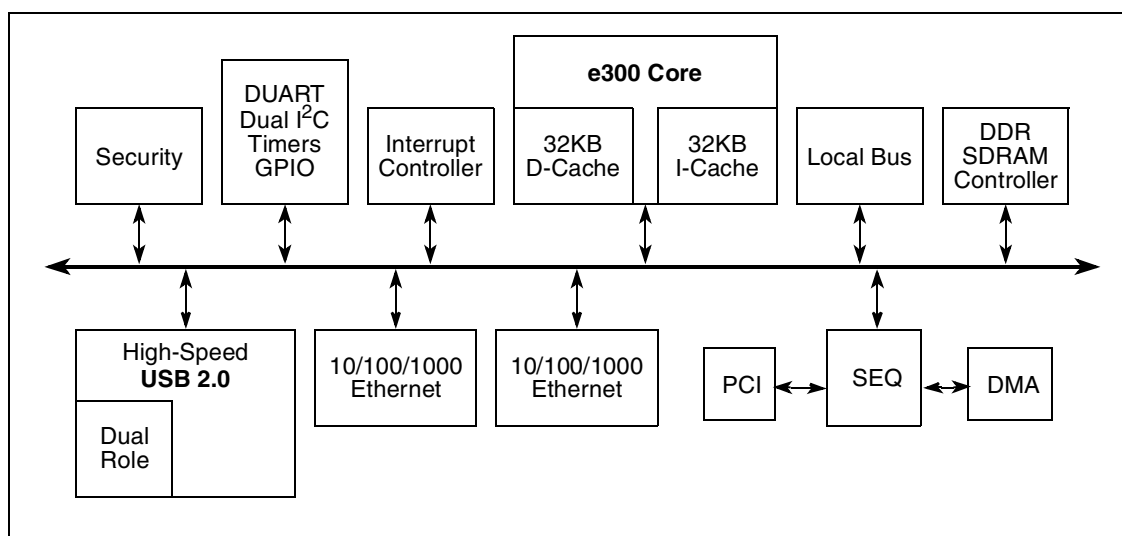
Figure 1. MPC8343EA Block Diagram
