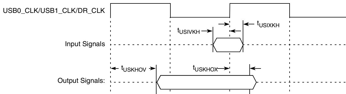
Figure 14. USB Signals
