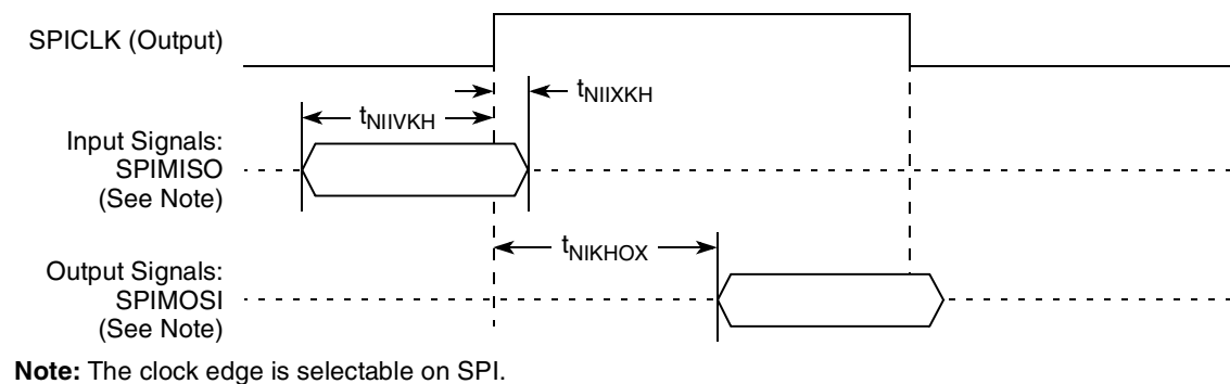
Figure 34. SPI AC Timing in Master Mode (Internal Clock) Diagram
