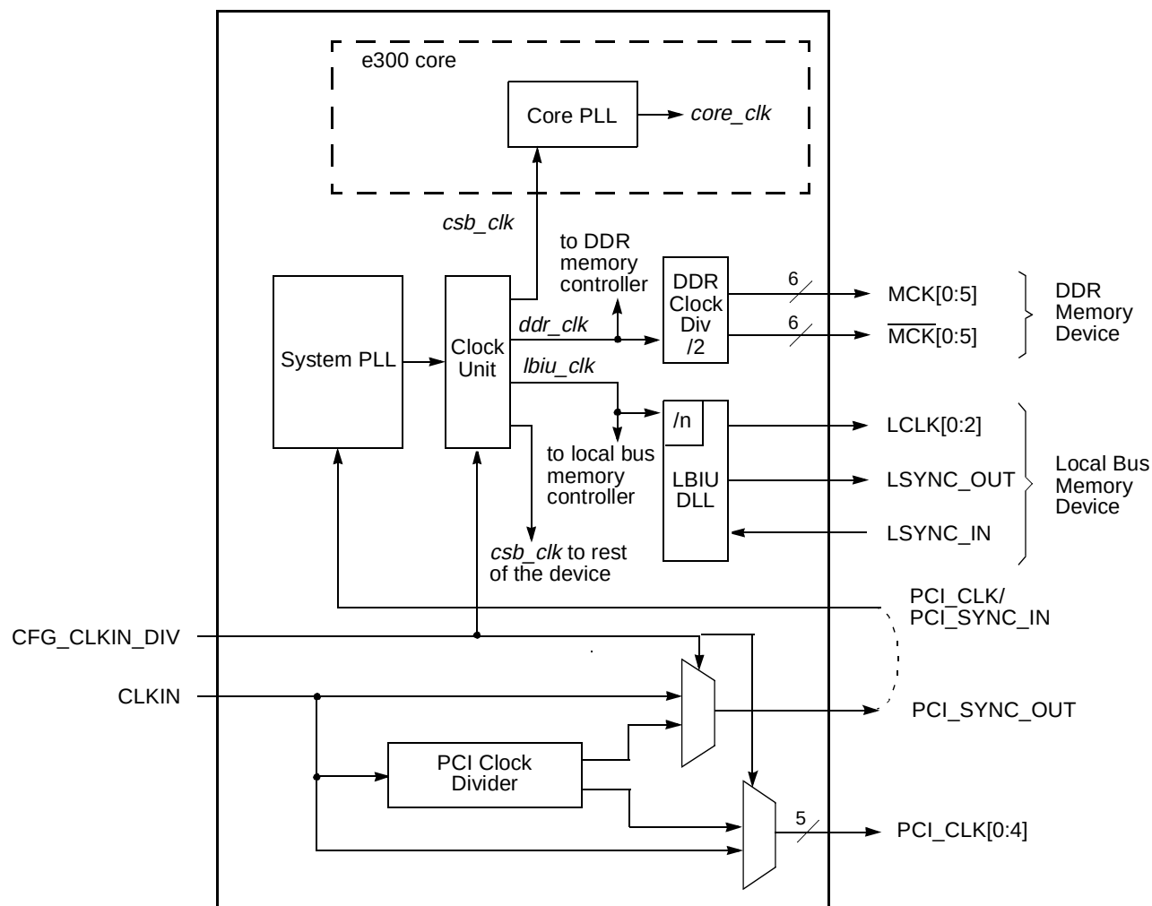
Figure 67. MPC8378E Clock Subsystem
