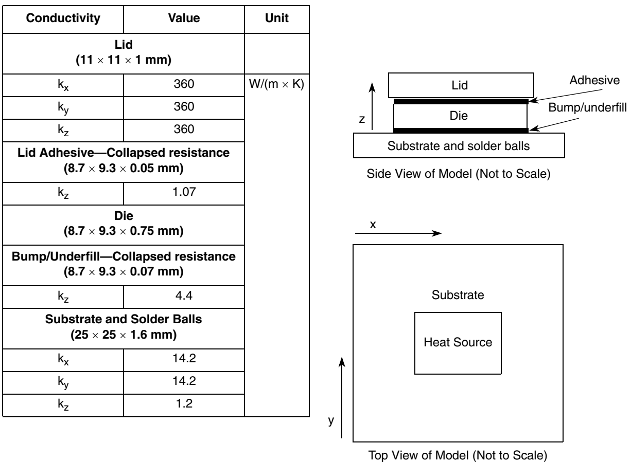
Figure 43. MPC8555E Thermal Model
