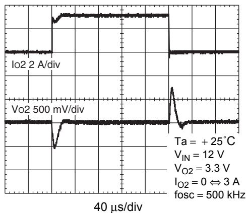
CH2 Sudden Load Variation Waveform
