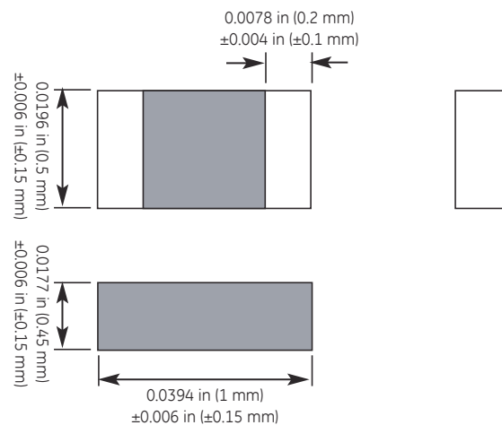
NTC Type NHQT Outline Drawing
