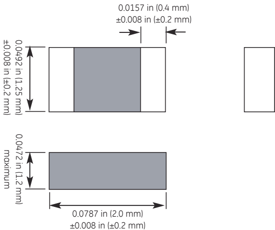
NTC Type NHQMM Outline Drawing
