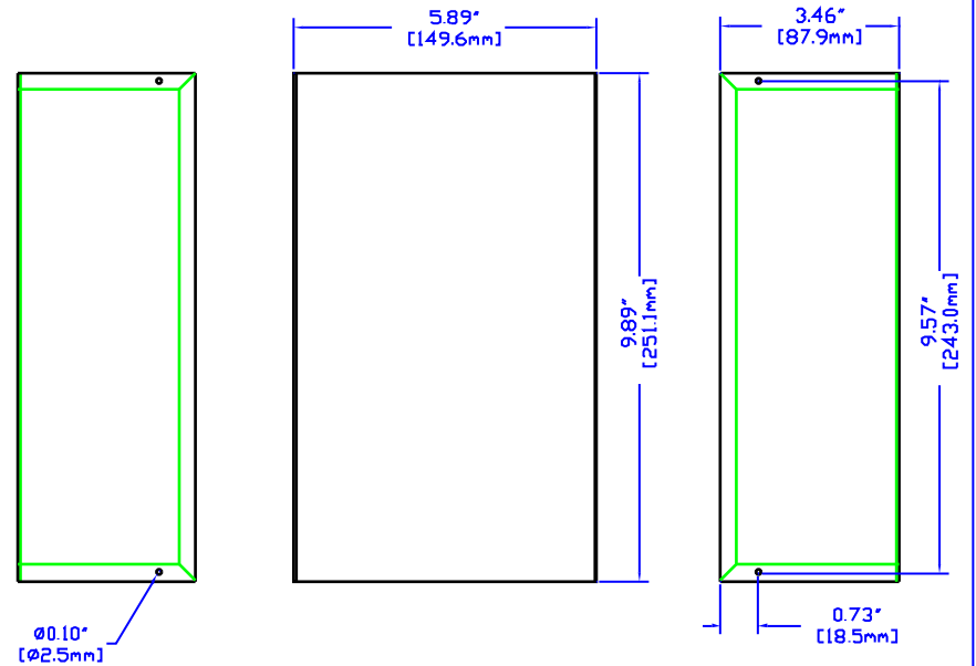
VIEW OF BASE <INSIDE>
