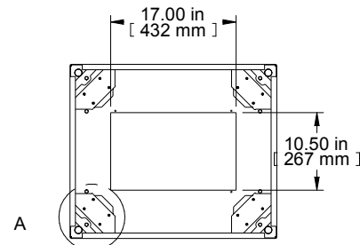
BOTTOM VIEW BOTTOM OPENING
