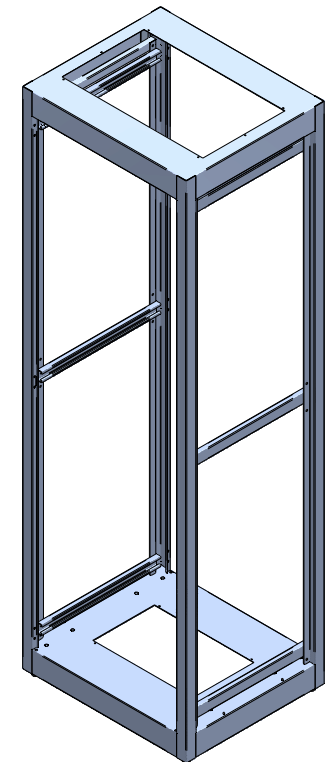
ISOMETRIC
