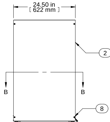
L.S. VIEW
