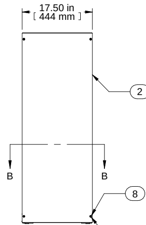
L.S. VIEW
