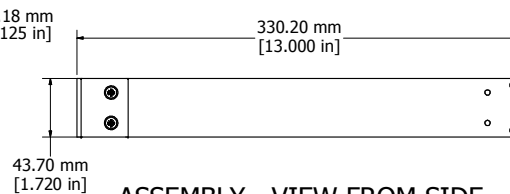
ASSEMBLY - VIEW FROM SIDE
