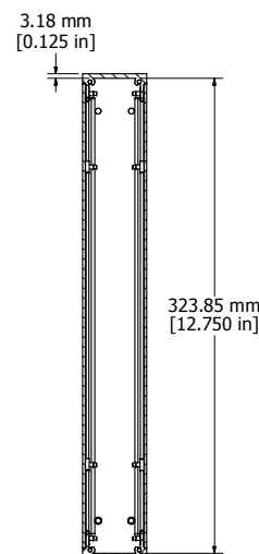
SECTION HH-HH
