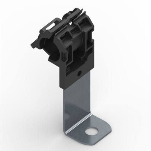
Ratchet P-Clamp, 0.52" - 0.77" Bundle Dia, 90° Long, .41" Hole Dia, PA66HIRHSUV/ST/ZN, Black, 200/ctn
