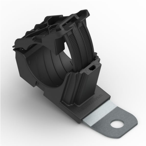
Ratchet P-Clamp, 0.76" - 1.42" Bundle Dia, 15° Short, .41" Hole Dia, PA66HIRHSUV/ST/ZN, Black, 160/ctn
