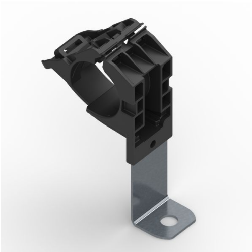
Ratchet P-Clamp, 0.76" - 1.42" Bundle Dia, 90° Long, .41" Hole Dia, PA66HIRHSUV/ST/ZN, Black, 140/ctn
