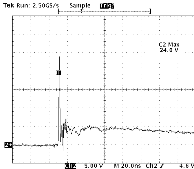
SMF12 ESD Clamping (8kV Contact per IEC 61000-4-2)
