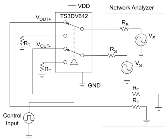
Figure 19. Differential Bandwidth (BW)
