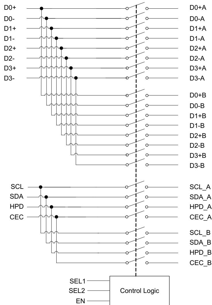
Figure 20. Logic Diagram
