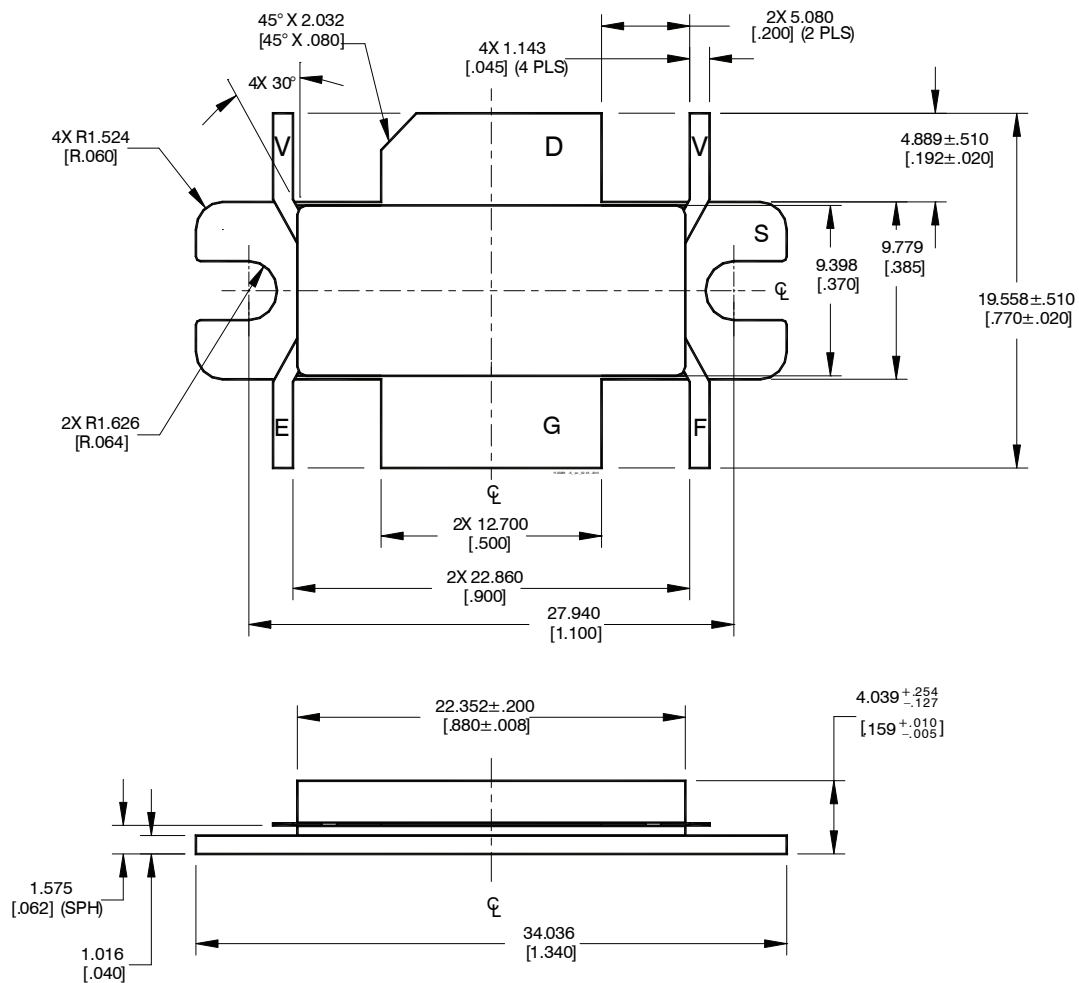
Package H-33288-6
