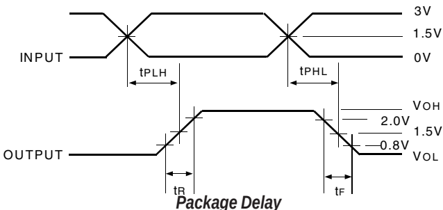
Package Delay
