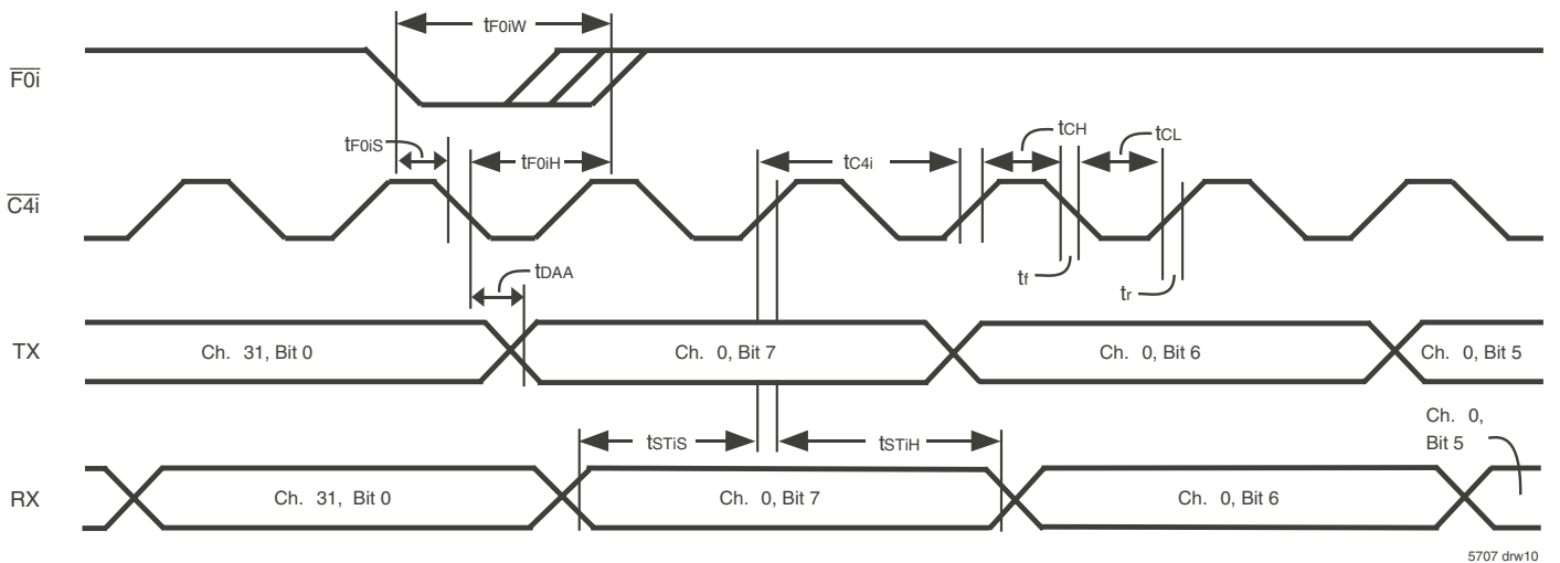
Figure 7. ST-BUS® Timing
