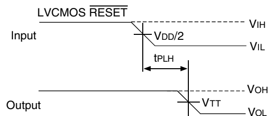
Voltage Waveforms - Propagation Delay Times with Respect to Reset Input
