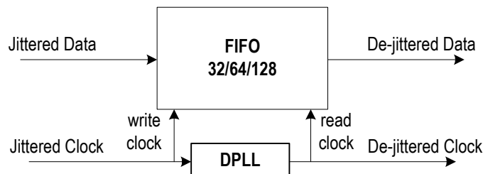
Figure-21 Jitter Attenuator
