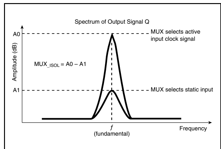
MUX_ISOLATION
