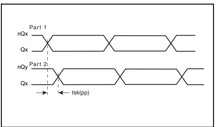
Part-to-Part Skew
