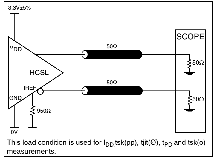
HCSSL Output Load AC Test Circuit
