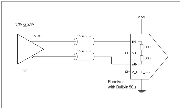
Figure 3A. IN/nIN Input with Built-In 50 \Omega Driven by an LVDS Driver
