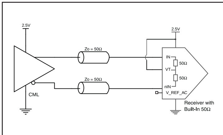
Figure 3C. IN/nIN Input with Built-In 50 \Omega Driven by a CML Driver
