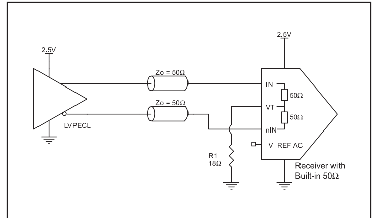
Figure 3B. IN/nIN Input with Built-In 50 \Omega Driven by an LVPECL Driver
