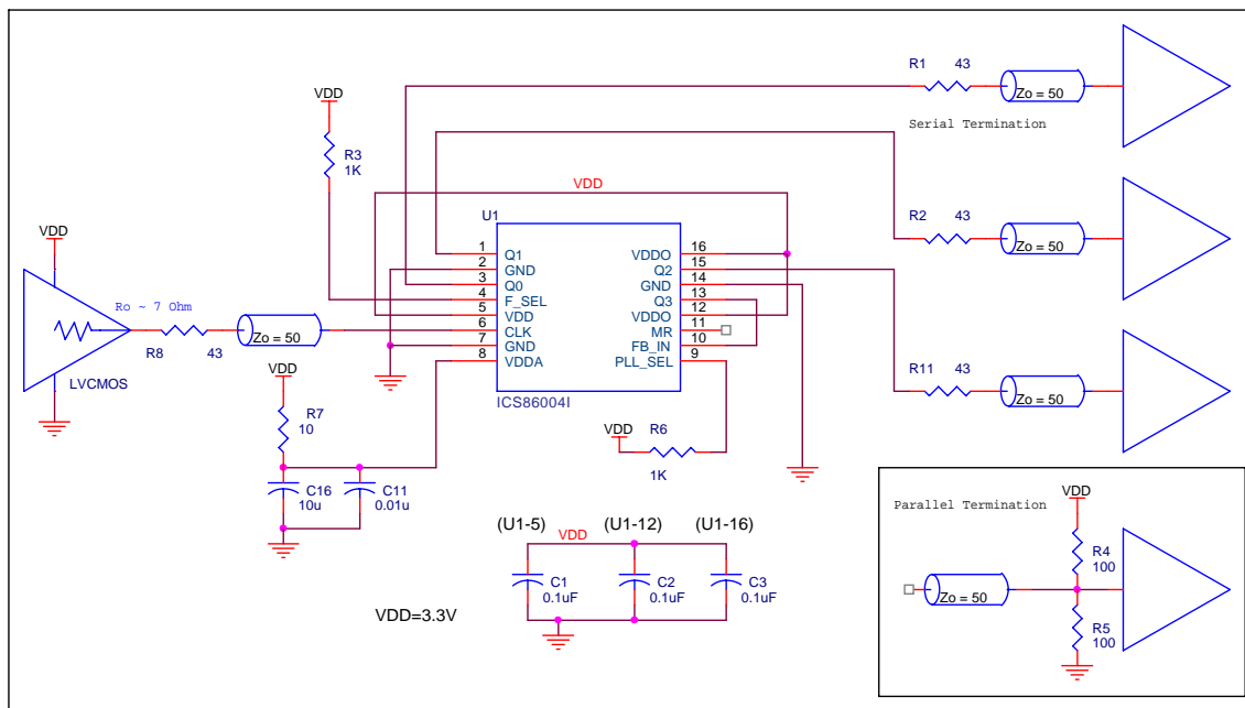
FIGURE 2. ICS86004I SCHEMATIC EXAMPLE
