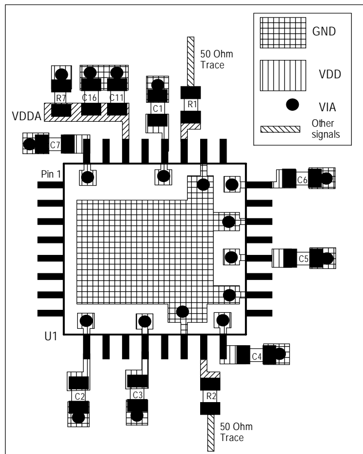
FIGURE 4B. PCB BOARD LAYOUT FOR ICS87051
