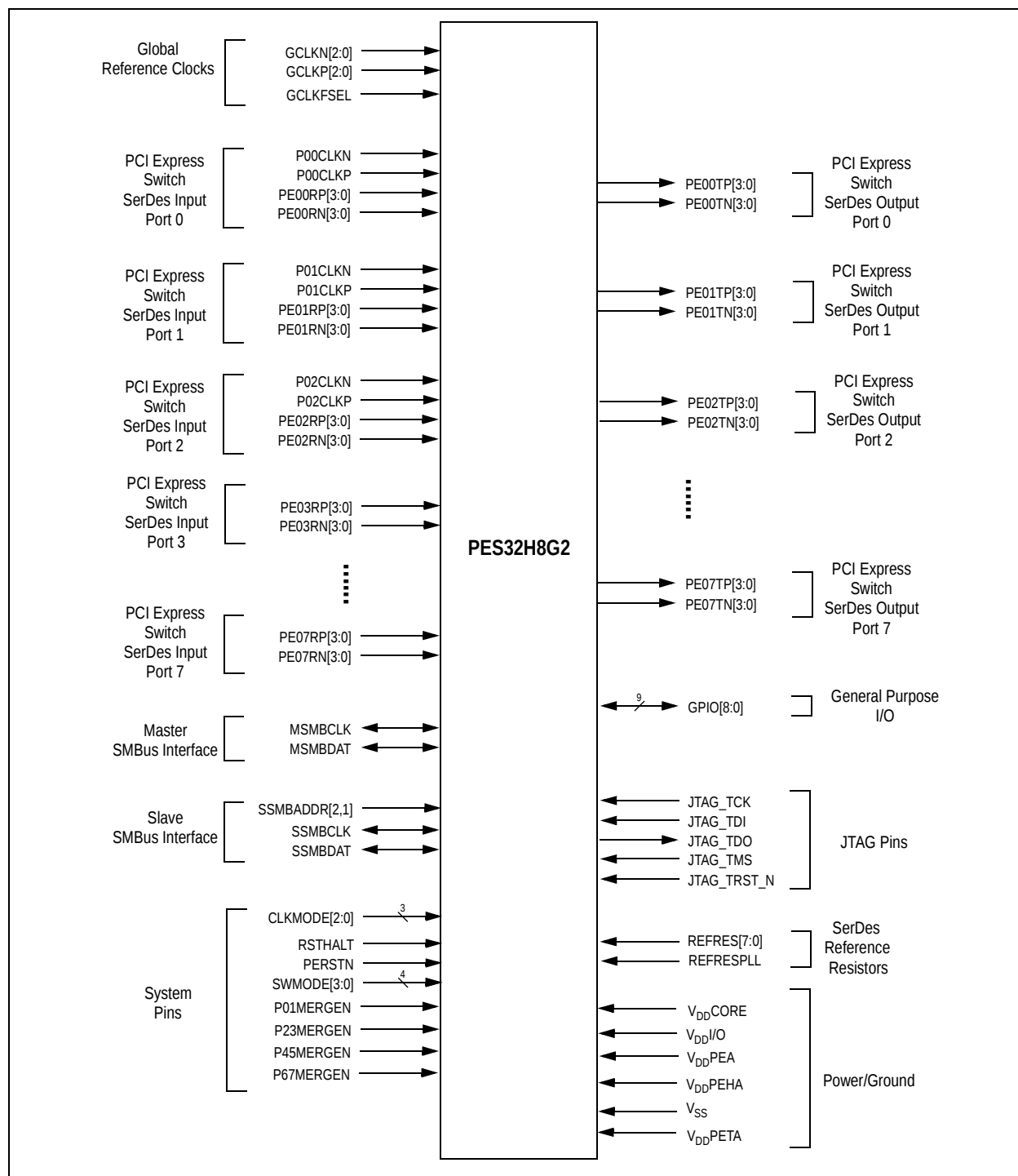
Figure 4 PES32H8G2 Logic Diagram
