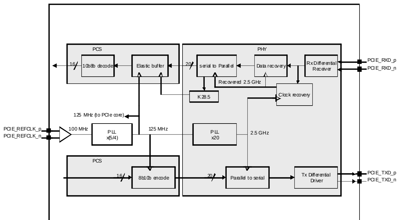
Figure 26: PCIe Clocking
