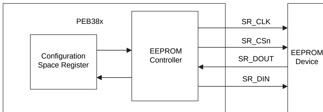
Figure 30: EEPROM Interface
