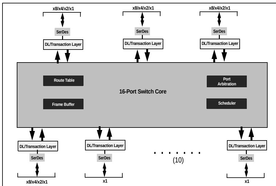
34 PCI Express Lanes Up to 6 x4 ports and 10 x1 Ports Figure 1 Internal Block Diagram
