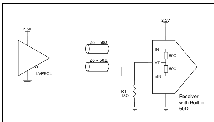
Figure 5B. IN/nIN Input with Built-In 50 \Omega Driven by an LVPECL Driver
