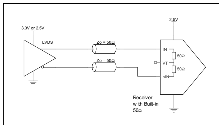
Figure 5A. IN/nIN Input with Built-In 50 \Omega Driven by an LVDS Driver
