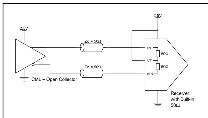
Figure 5C. IN/nIN Input with Built-In 50 \Omega Driven by a CML Driver
