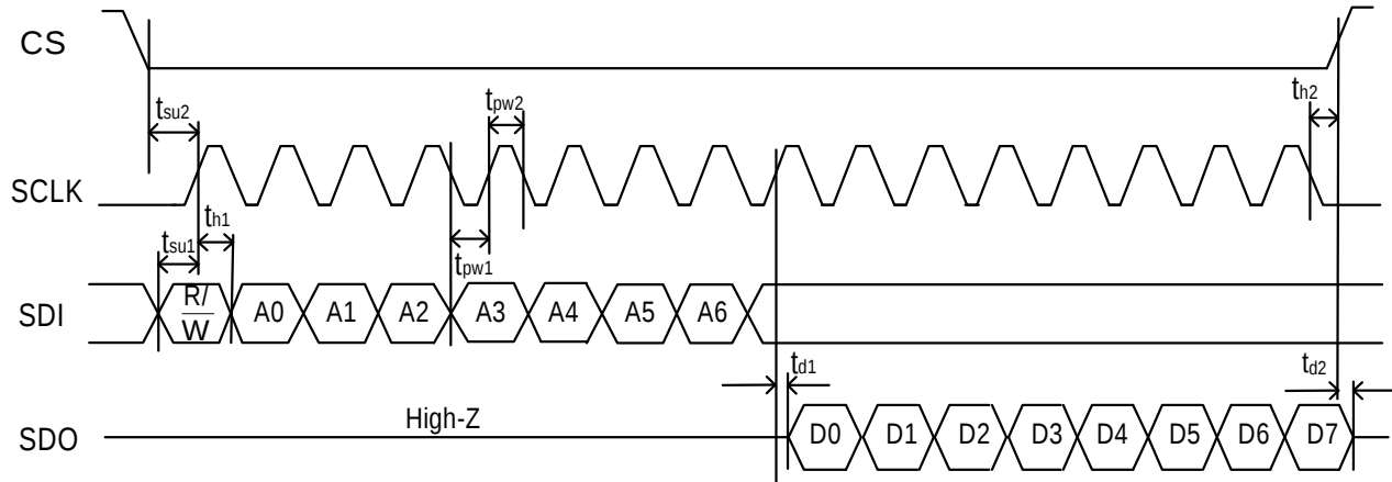
Figure 9. Serial Read Timing Diagram (CLKE Asserted Low)
