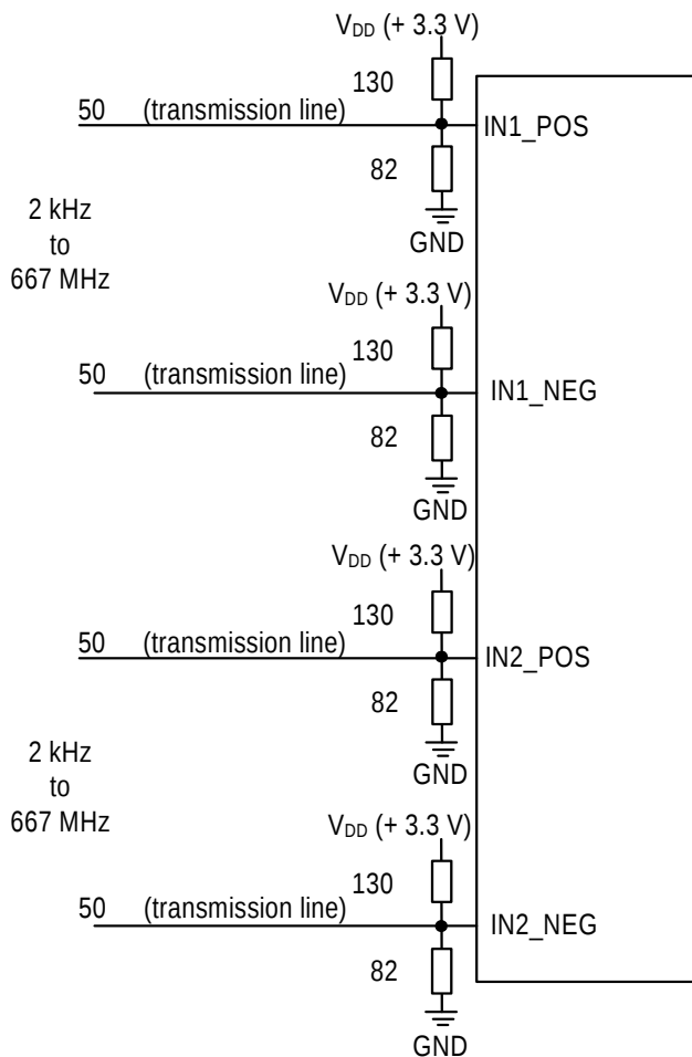
Figure 15. Recommended PECL Input Port Line Termination
