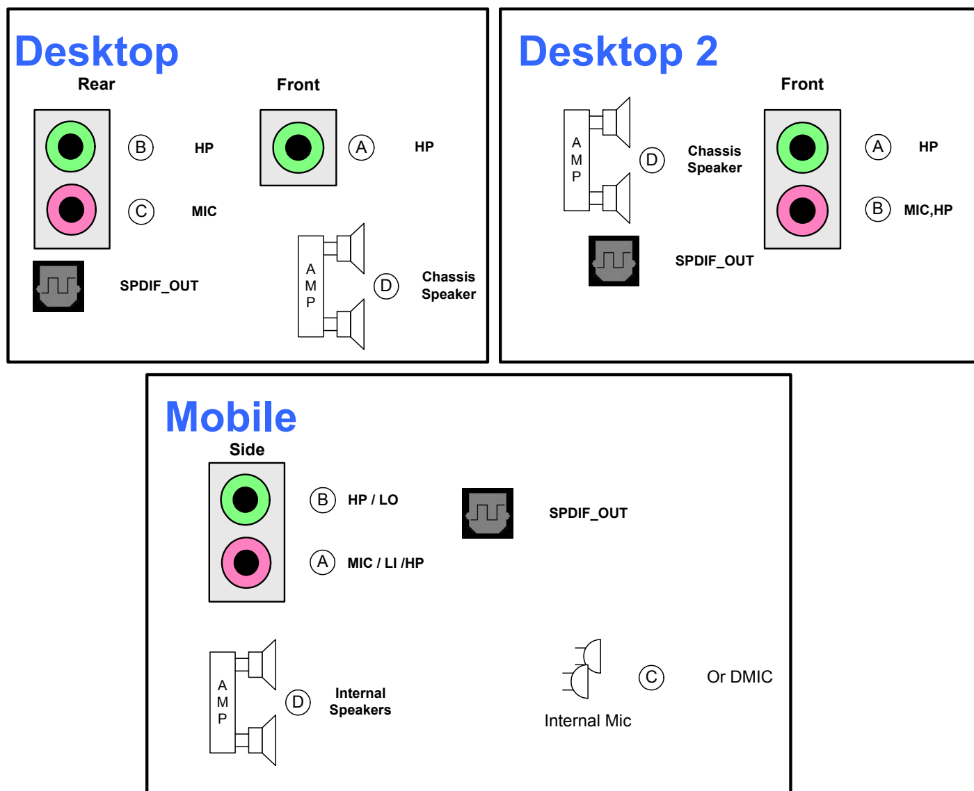
Figure 14. Port Configurations
