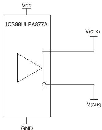
Figure 1: IBIS Model Output Load
