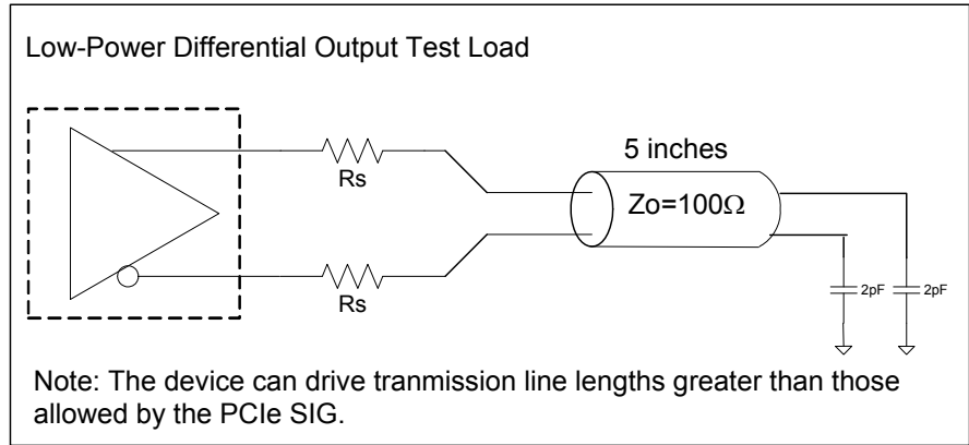
Alternate Differential Output Terminations
