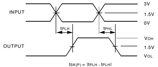
Pulse Skew
