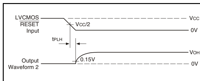
Voltage Waveforms: Open Drain Output Low-to-High Transition Time (with respect to \overline{\text{RESET}} input)
