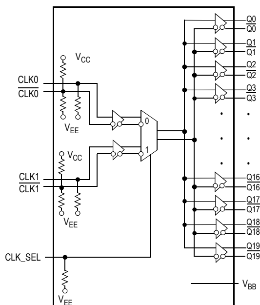
Figure 1. MC100ES6221 Logic Diagram
