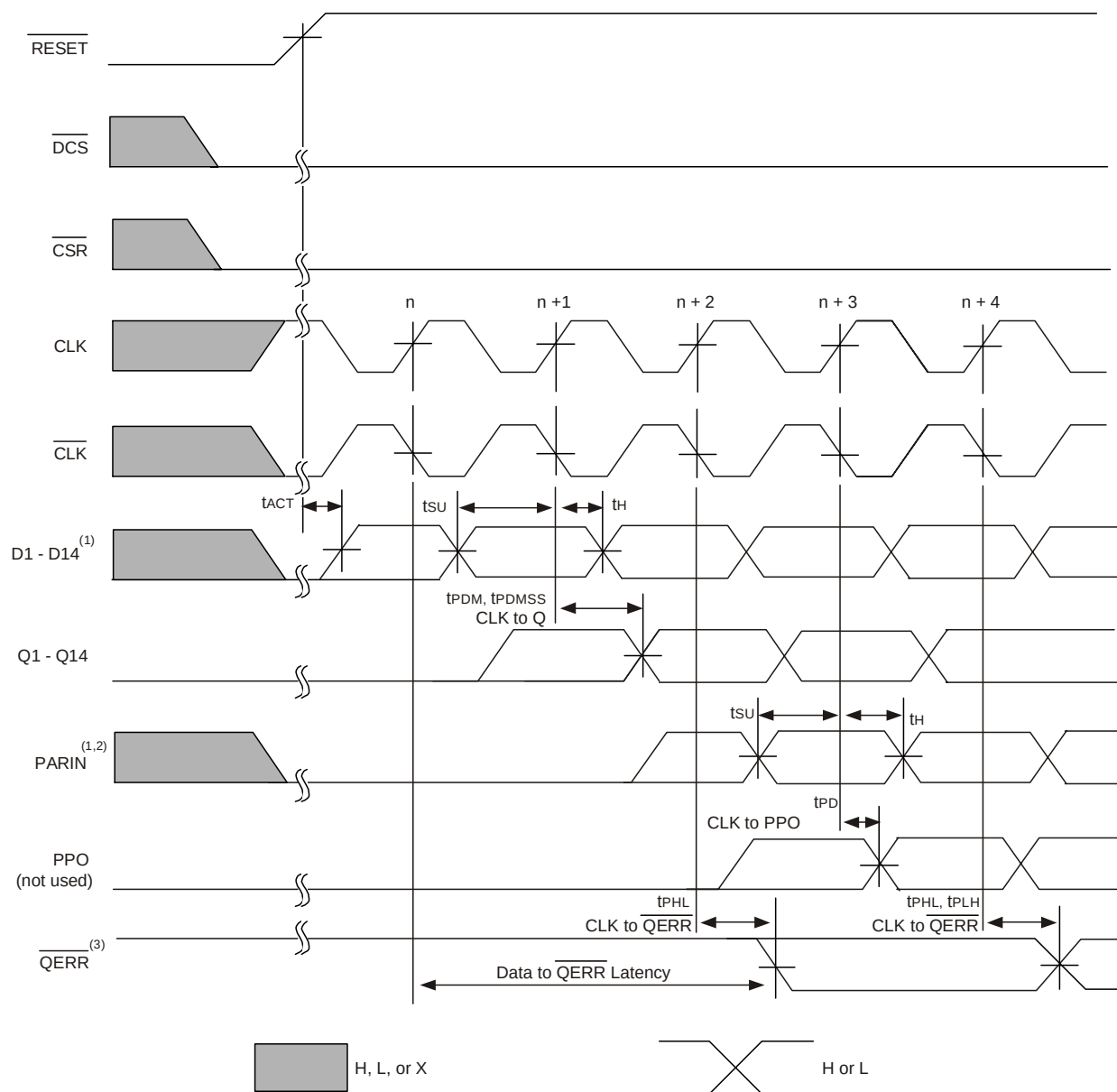
Timing Diagram for the Second SSTUAF32866C (1:2 Register-B Configuration) Device Used in a Pair; \text{C0} = 1 , \text{C1} = 1 , \overline{\text{RESET}} Switches from L to H
