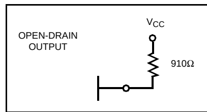
Figure 5. Connection Recommendation for \overline{LOCK}
