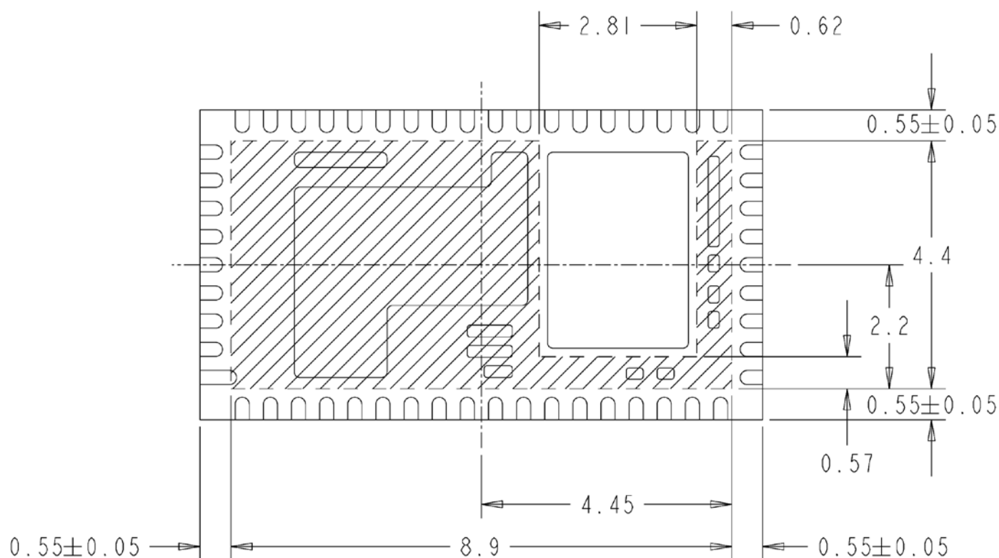
Shaded area highlights exposed metal that is not to be mechanically or electrically connected to the PCB.
