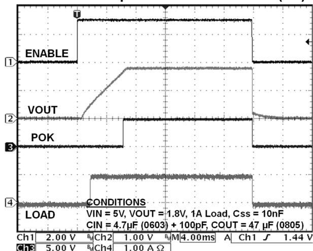
Enable Startup/Shutdown Waveform (1A)
