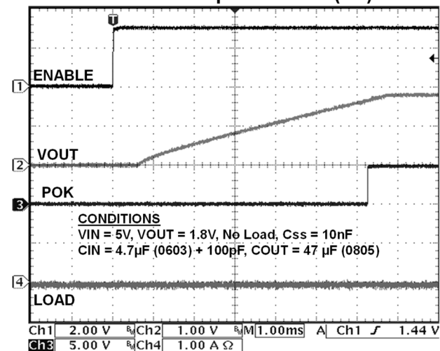
Enable Startup Waveform (0A)
