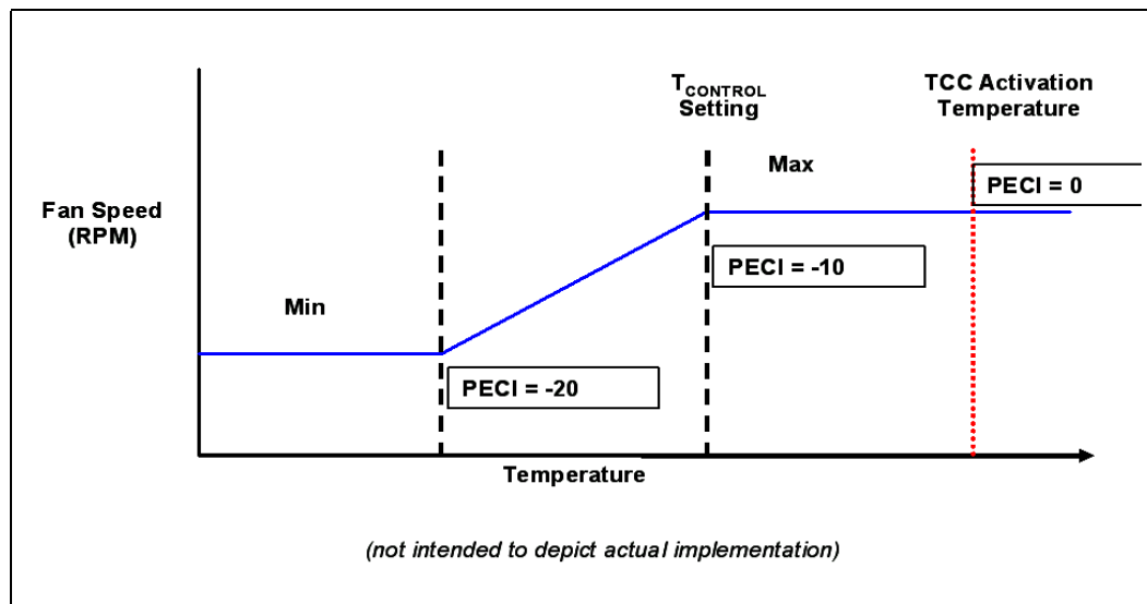
Figure 5-4. Conceptual Fan Control Diagram on PECI-Based Platforms
