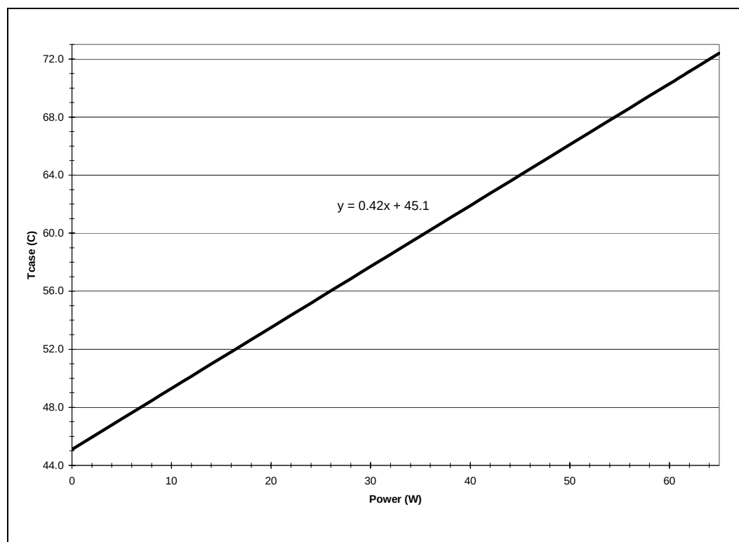
Figure 5-1. Processor Thermal Profile
