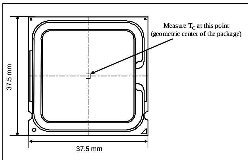
Figure 5-2. Case Temperature ( T_C ) Measurement Location
