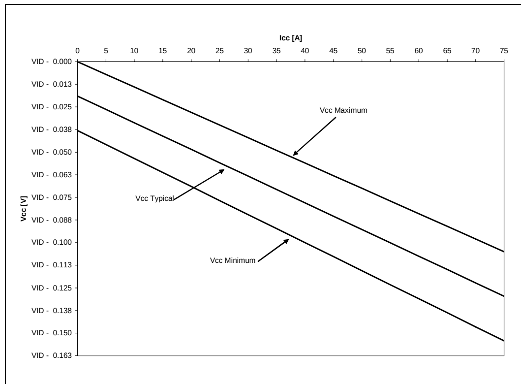
Figure 2-1. Processor V CC Static and Transient Tolerance
