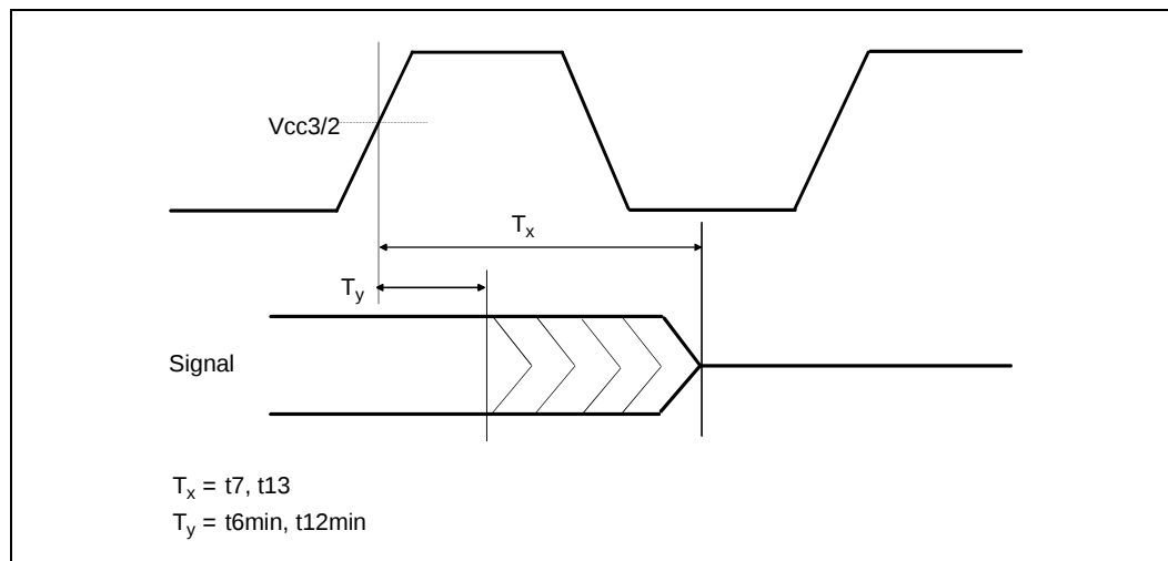
Figure 15. Float Delay Timings
