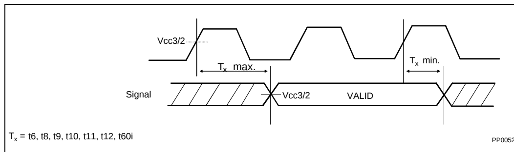
Figure 15. Float Delay Timings
