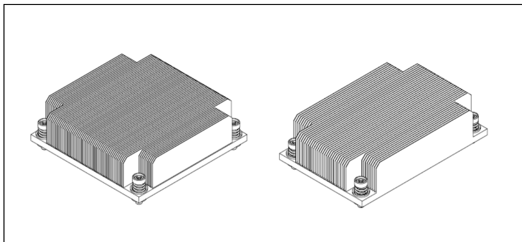
Figure 10-3. STS200P and STS200PNRW 25.5 mm Tall Passive Heat Sinks
